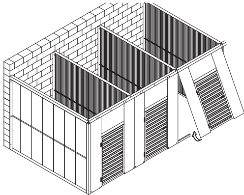
CORRUGATED SWING DOOR DETAIL
