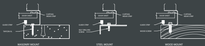
GUIDE MOUNTING
