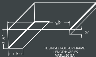
Single Roll Up Frame
