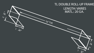
Double Roll Up Frame
