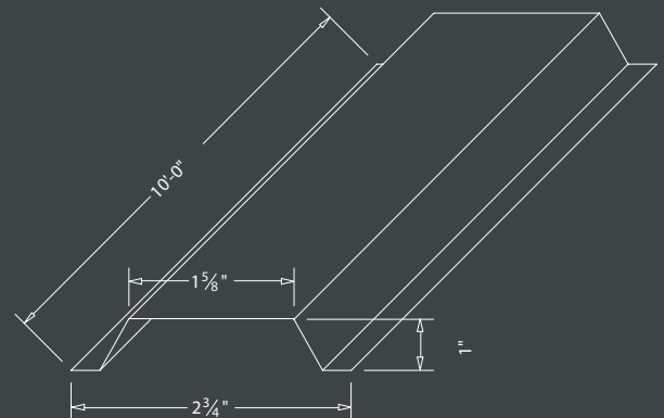
BURGLAR BAR DETAIL
