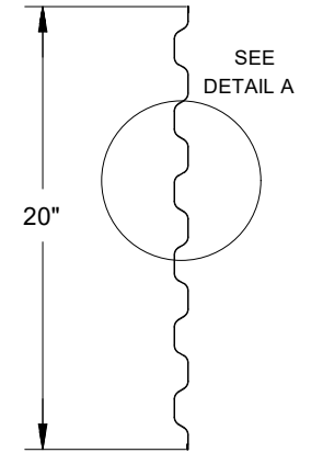
26 GA CURTAIN PANEL DETAIL
