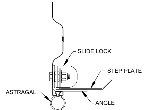
BOTTOM BAR ASSEMBLY
