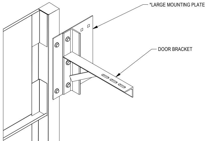
FIGURE 7: DOOR BRACKET TO MOUNTING PLATE
