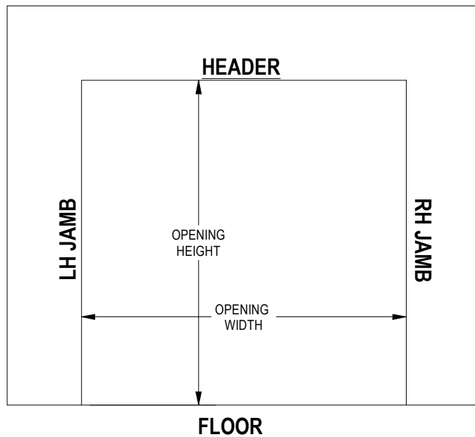
FIGURE 4: WALL OPENING
