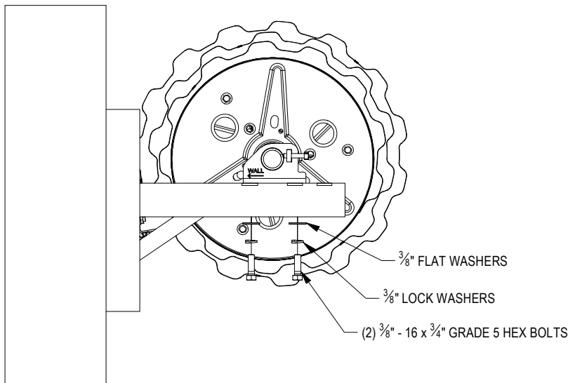
FIGURE 17: SECURING STAMPED AXLE SUPPORT TO BRACKETS
