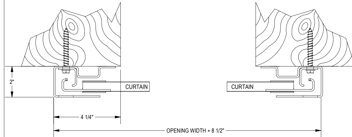
FIGURE 14: WOOD JAMBS
