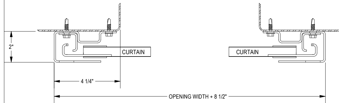
FIGURE 15: STEEL JAMBS
