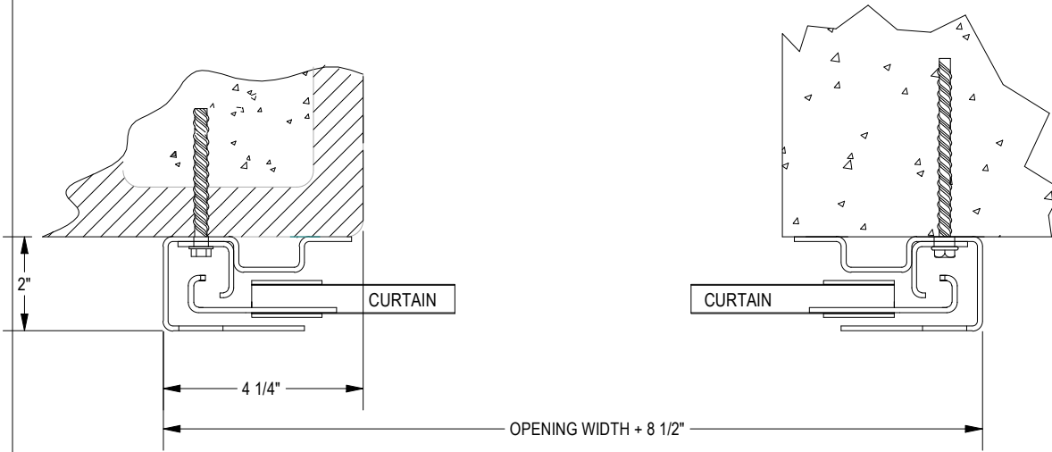
FIGURE 13: CONCRETE / MASONRY JAMBS
