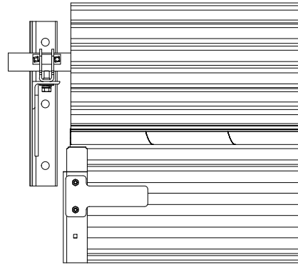
FIGURE 22: HEADSTOPS
