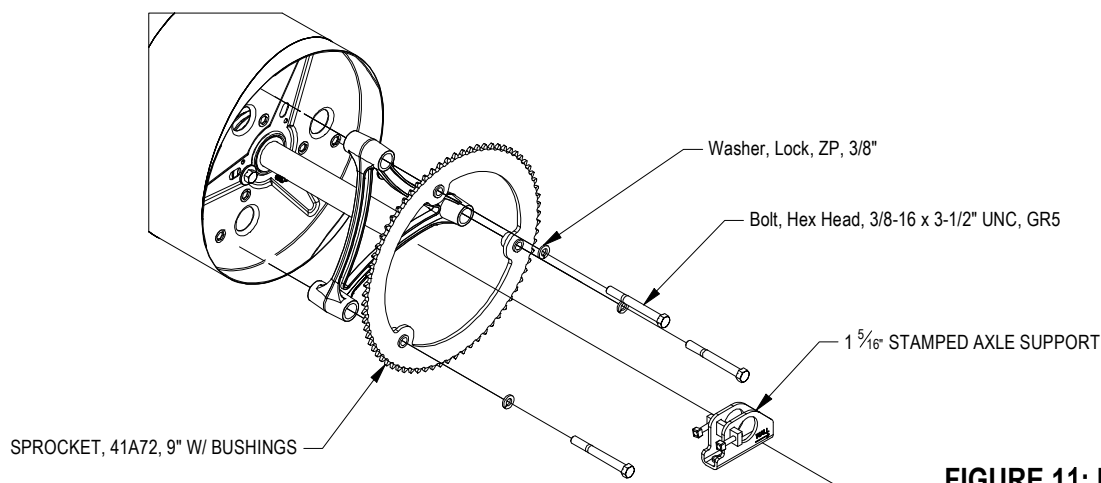
FIGURE 11: ELECTRIC OPERATOR
