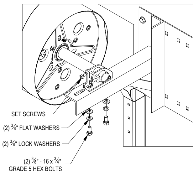
FIGURE 13: SECURING SADDLE
