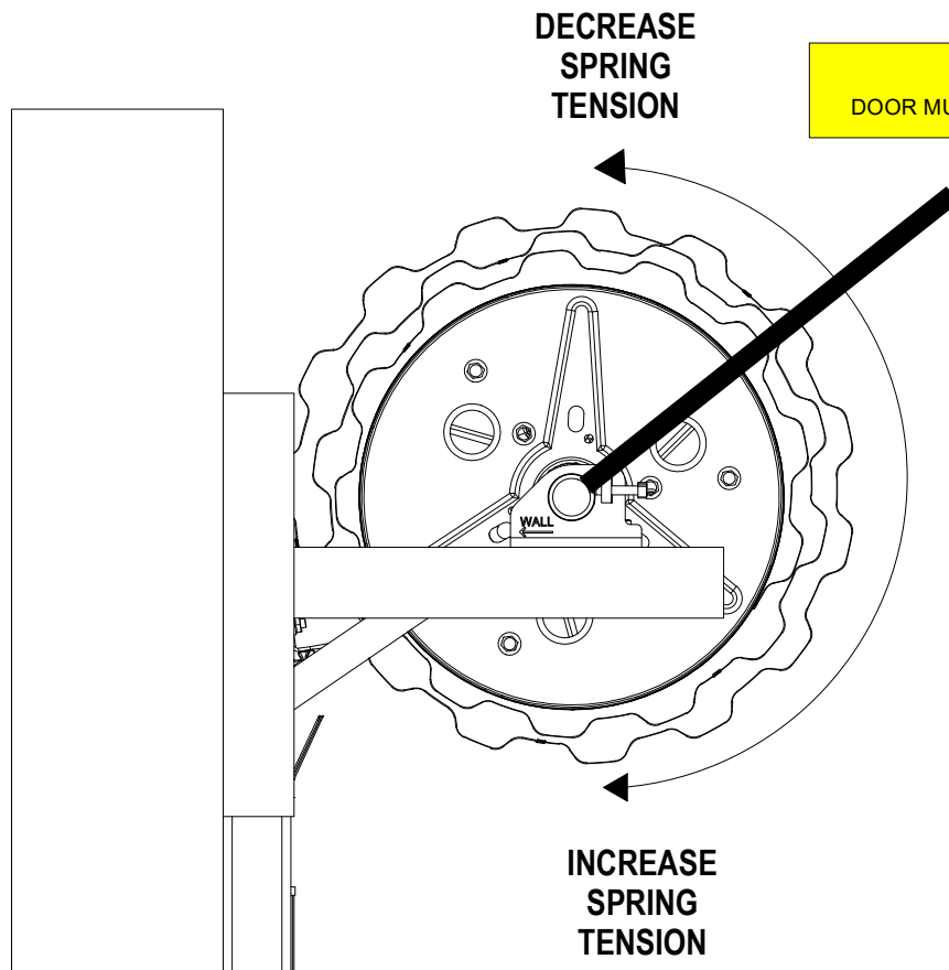
FIGURE 24: ADJUST SPRING TENSION
