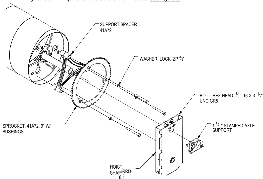
FIGURE 9: CHAIN HOIST 8:1
