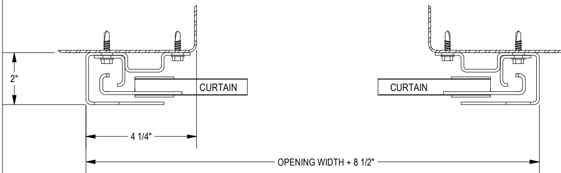
FIGURE 14: STEEL JAMBS
